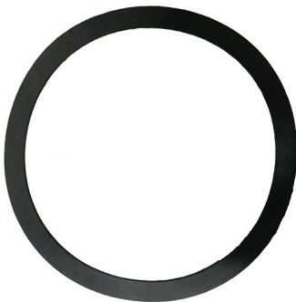
1000-6427 GASKETS 10.125" OD 8.75" ID .250" Thick For Guardian 3" and 4" H & L Strainers
